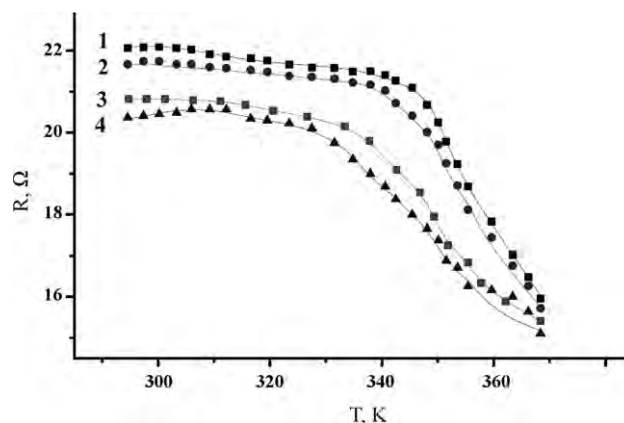
Fig. 8. Resistance as a function of temperature for a \text{La}_{0.775}\text{Sr}_{0.225}\text{MnO}_3 film on a \text{Ba}_{0.996}\text{Y}_{0.004}\text{TiO}_3 substrate in applied electric (between the electrodes 1 and 2) and magnetic fields: H = 1.2 \text{ MA/m} , V = 0 (1); H = 1.2 \text{ MA/m} , V = 20 \text{ V} (2); H = 0 , V = 0 (3); H = 0 , V = 20 \text{ V} (4).
